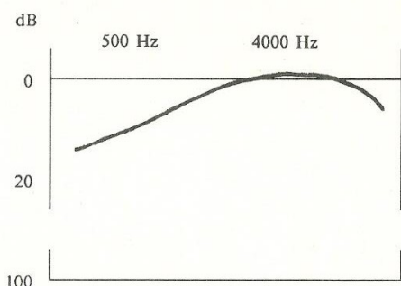
Fig. 1 - The specific threshold curve of the musical ear (from Tomatis, 1963, p.101)
