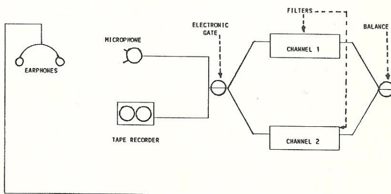
Fig. 2 - Diagram of the Electronic Ear
